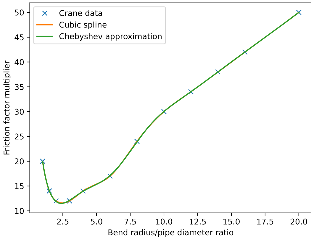
Interpolation of Crane ft multipliers for pipe bend losses
